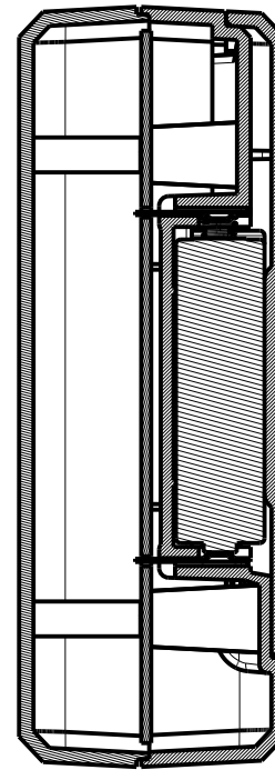
SECTION X-X
