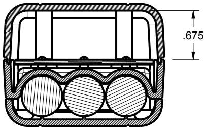
SECTION Y-Y
